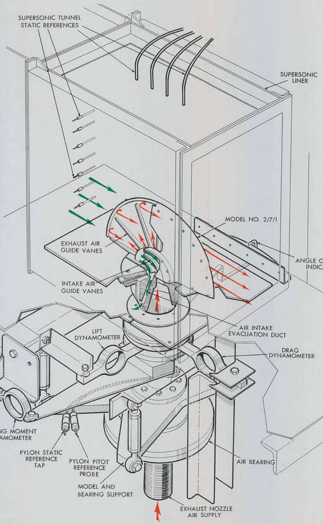
STABILITY AND CONTROL MODELS NO. 2/5, 2/6 AND 2/7
